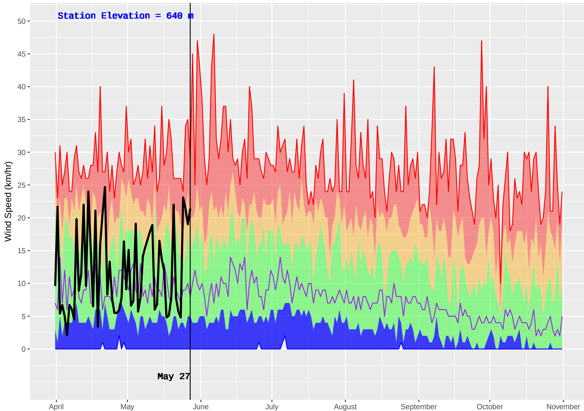
MERRITT HUB (294) : Historical (1978–2016) and Current (2018) Noon Wind Speed
